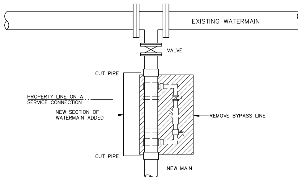
FINAL CONNECTION OF NEW WATERMAIN TO EXISTING WATERMAIN
